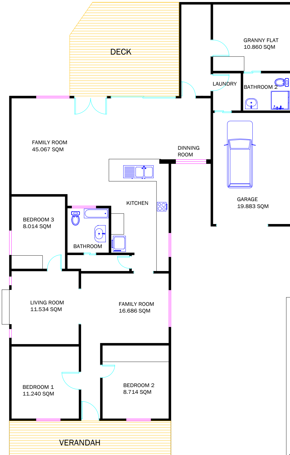
Floor Plan
